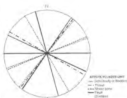
Figure 11. Rose Diagram of tectonic elements.
