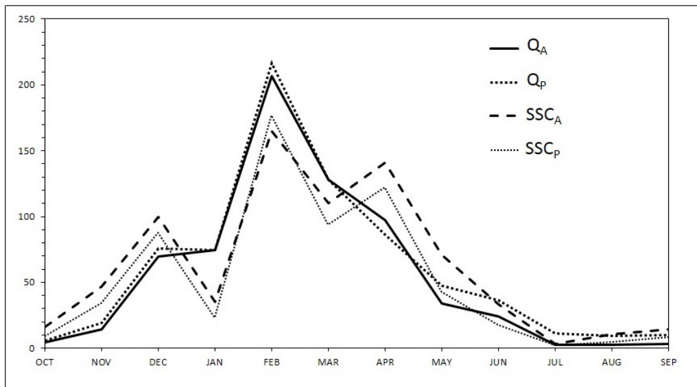
Figure 5. Monthly variations of water flow ( \text{m}^3/\text{s} ) and SSC ( \text{mg/L} ) [Q: flow; (A): Agia Paraskevi and (P): PalaioPyrgos]
