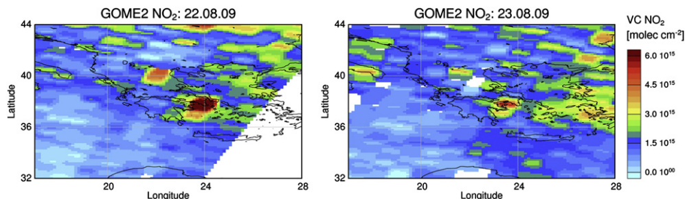
Fig. 3. GOME-2 Vertical Column Densities of NO 2 over Greece. The highest values of VCD NO 2 (shown in red) were obtained on August 22 and 23. (For interpretation of the references to color in this figure legend, the reader is referred to the web version of this article.)
