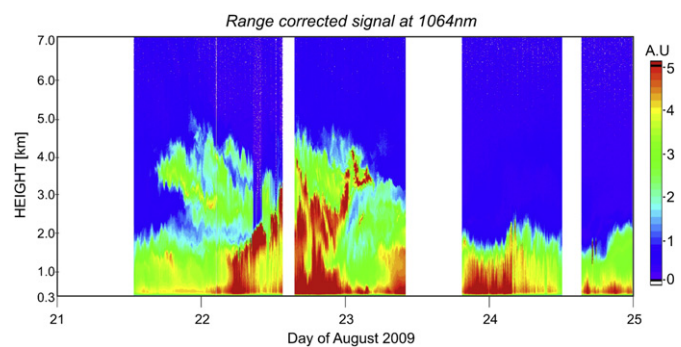
Fig. 5. Time-series of the range-corrected backscatter signal vertical distribution at 1064 nm (Arbitrary Units – A.U.) from 21 to 25 August 2009. The vertical and temporal resolution is of the order of 15 m and 90 s, respectively.
