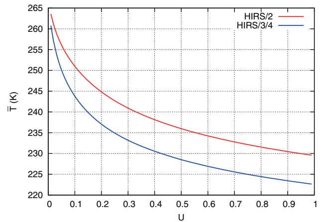
Figure 3: Mean emission temperatures for HIRS/2 (6.7 μm) and HIRS/3/4 (6.5 μm) water vapour channels, as a function of upper tropospheric humidity. The mean temperature of emission decreases with increasing U . Differences between HIRS/2 and HIRS3/4 curves are the order of 7 K.
