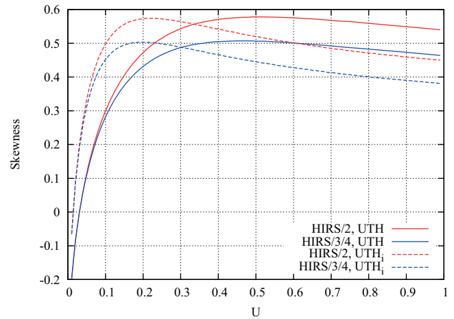
Figure 2: Skewness of the distribution functions of emission pressure levels for UTH and UTH i and for HIRS/2 (6.7 μm) and HIRS/3/4 (6.5 μm) water vapour channels, as a function of upper tropospheric humidity. Except for very dry situations the distributions have a tail to higher pressures (positive skewness).
