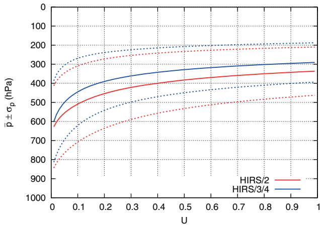
Figure 1: Mean emission pressure levels (solid) and their standard deviations (dashed) for HIRS/2 (6.7 μm) and HIRS/3/4 (6.5 μm) water vapour channels, as a function of upper tropospheric humidity. The mean height of emission has little dependence on U for U > 50\% .
