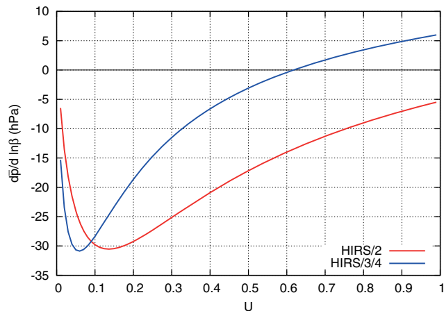
Figure 6: The derivative of mean emission pressure to relative change of the lapse rate parameter \beta at its standard value \beta = 0.22 for HIRS/2 (6.7 \mu\text{m} ) and HIRS/3/4 (6.5 \mu\text{m} ) water vapour channels, as a function of upper tropospheric humidity. A ten-percent change of \beta from its standard value thus implies an absolute pressure change of less than about 3 hPa.
